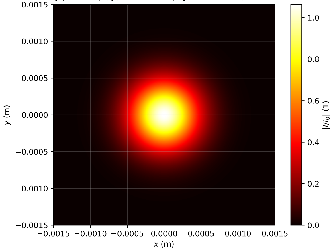
Intensity profile I(x, y, z = 0.398m)/I_0 , P_{in}=0.7P_{cr} , artificial time
